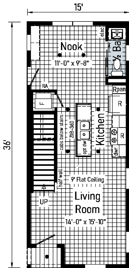
Main Floor
