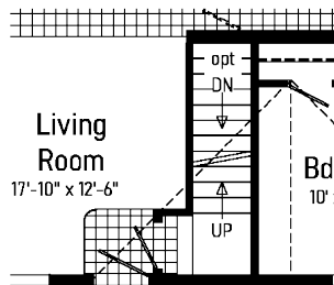
Opt Attic Stairs
