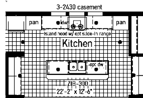
Alternate Kitchen w/ Opt Casement Windows
