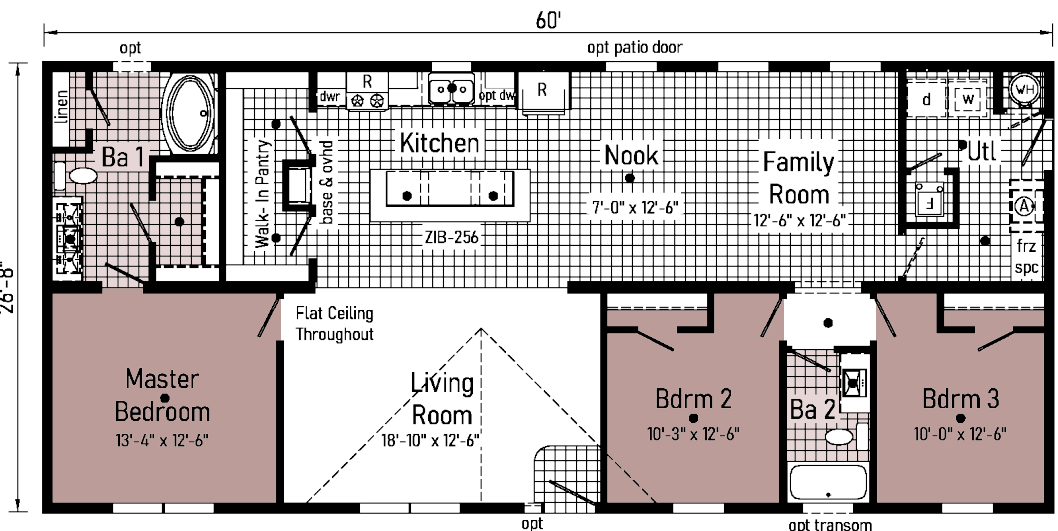
Alternate Walk-In Pantry & Master Closet
