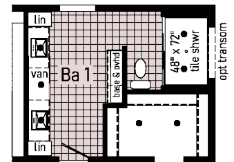
Optional 4' x 6' Walk-In Tile Shower
