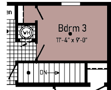
Optional Stairwell (omits base & overhead)
