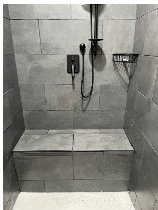
Ceramic Bench For 4x8 Shower Requires Ceramic Floor
